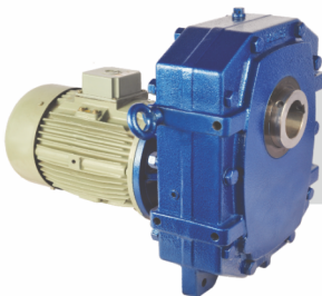
Parellet Helical Geared Motor
